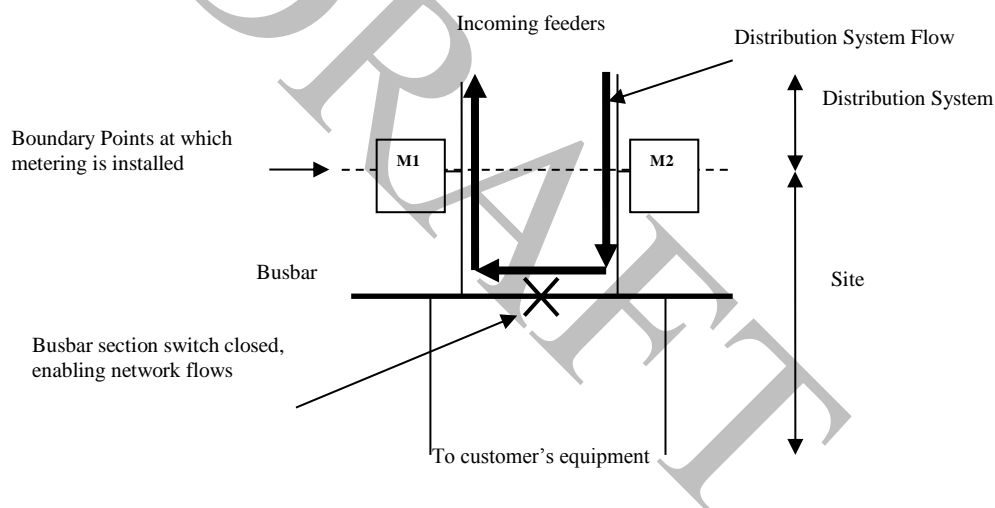
Figure 1. Distribution Network Flows
