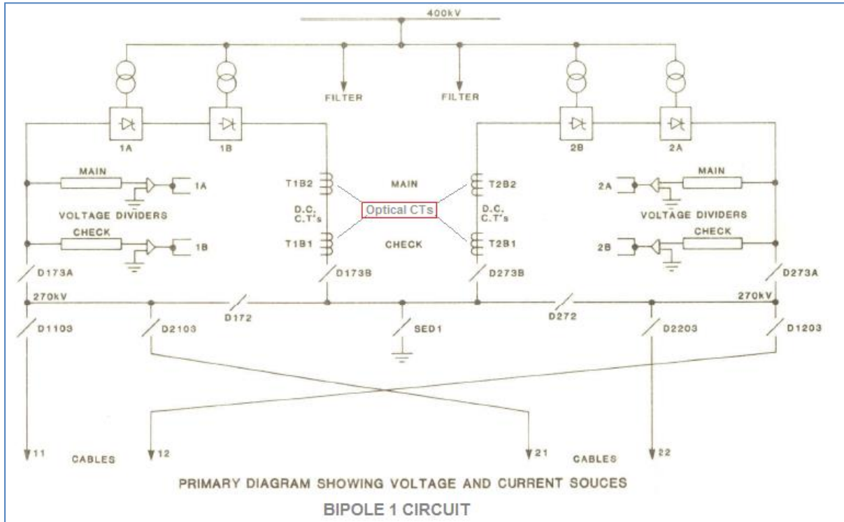
Figure 1 – Bipole 1 metering Current and Voltage measuring positions.
